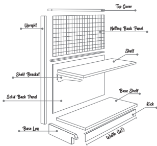
Wall Gondola (Single Side) Run along the wall.
